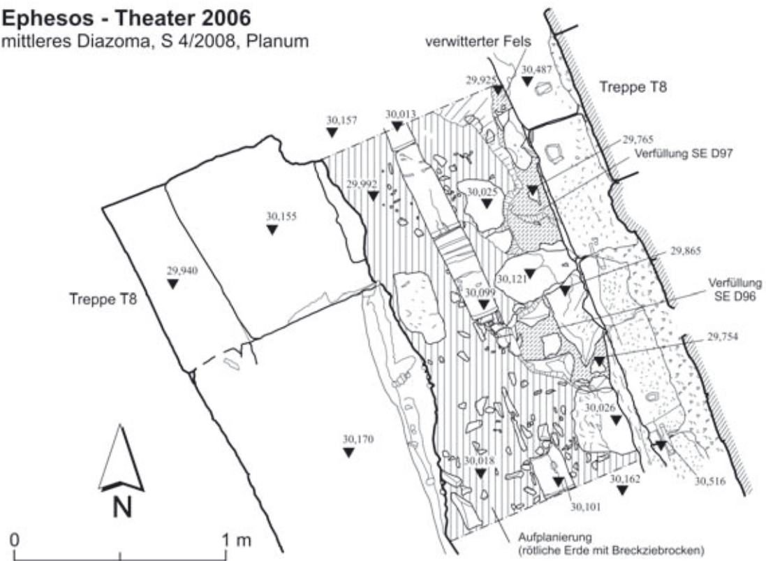
Abb. 231: Mittleres Diazoma, S 4/2008, Planum
